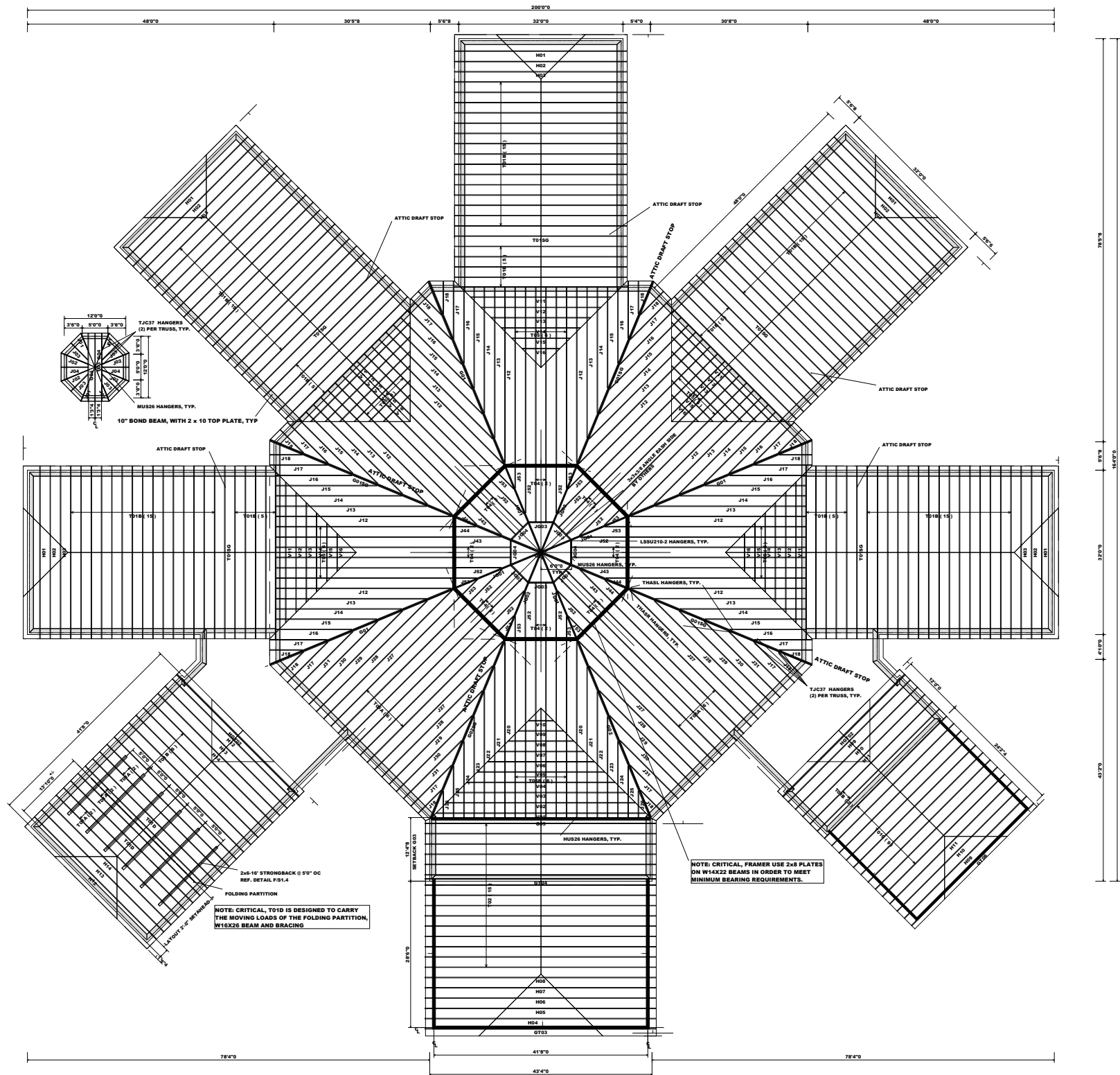
TRUSS PLACEMENT LAYOUT
